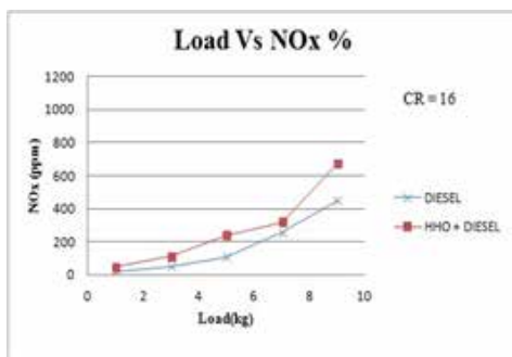
Figure 12 Load Vs NOx at CR 16
