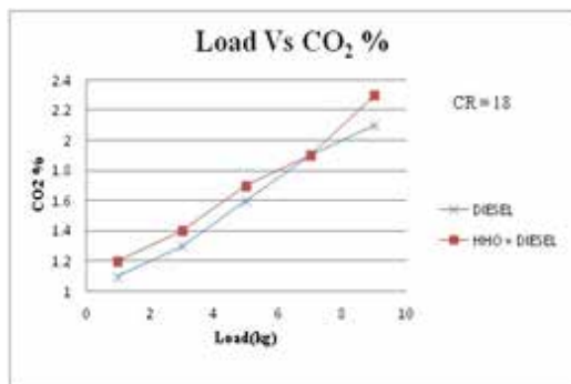
Figure 11 Load Vs CO2 at CR 18
