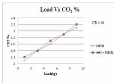
Figure 9 Load Vs CO2 at CR 16
