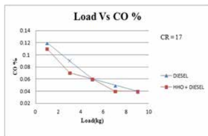
Figure 4 Load Vs CO at CR 17
