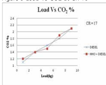
Figure 10 Load Vs CO2 at CR 17
