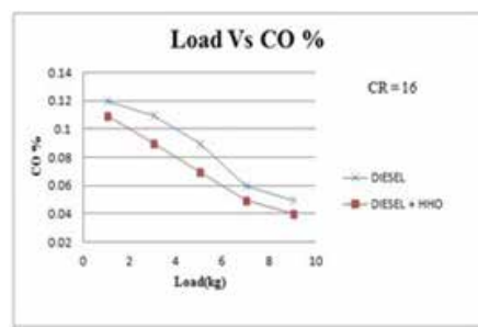
Figure 3 Load Vs CO at CR 16
