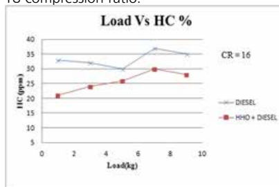
Figure 6 Load Vs HC at CR 16
