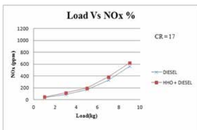
Figure 13 Load Vs NOx at CR 17
