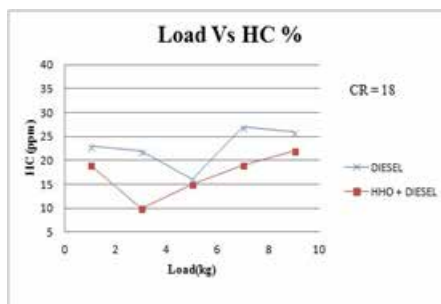
Figure 8 Load Vs HC at CR 18
