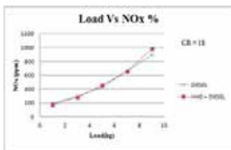
Figure 14 Load Vs NOx at CR 18
