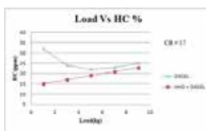
Figure 7 Load Vs HC at CR 17
