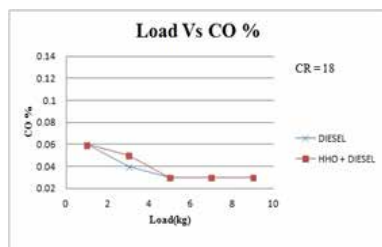
Figure 5 Load Vs CO at CR 18
